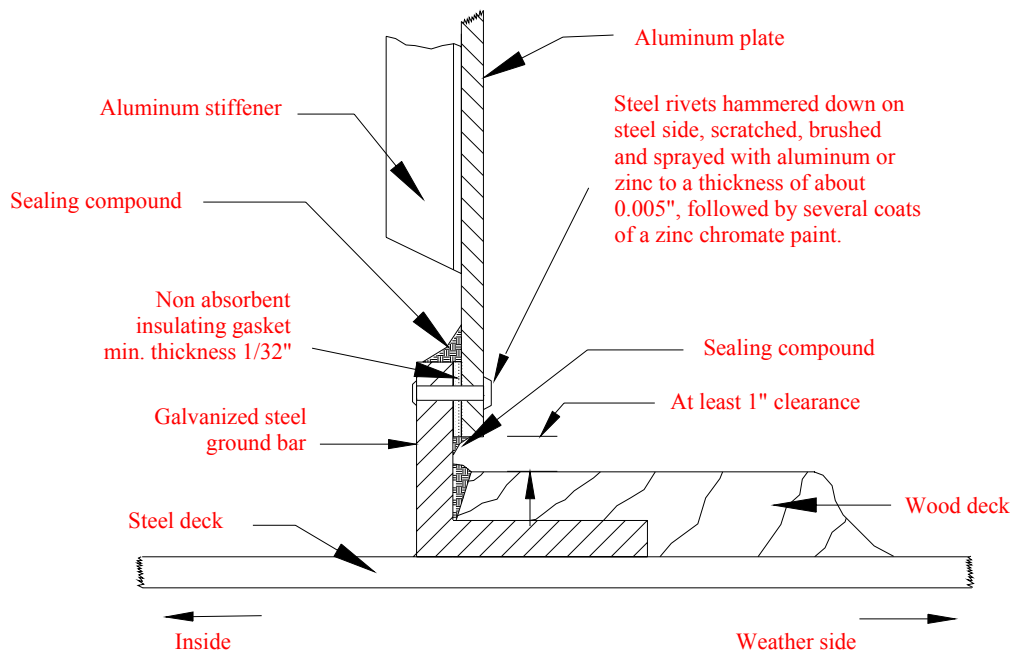
FIGURE 1 – CONNECTIONS OF DISSIMILAR METALS
